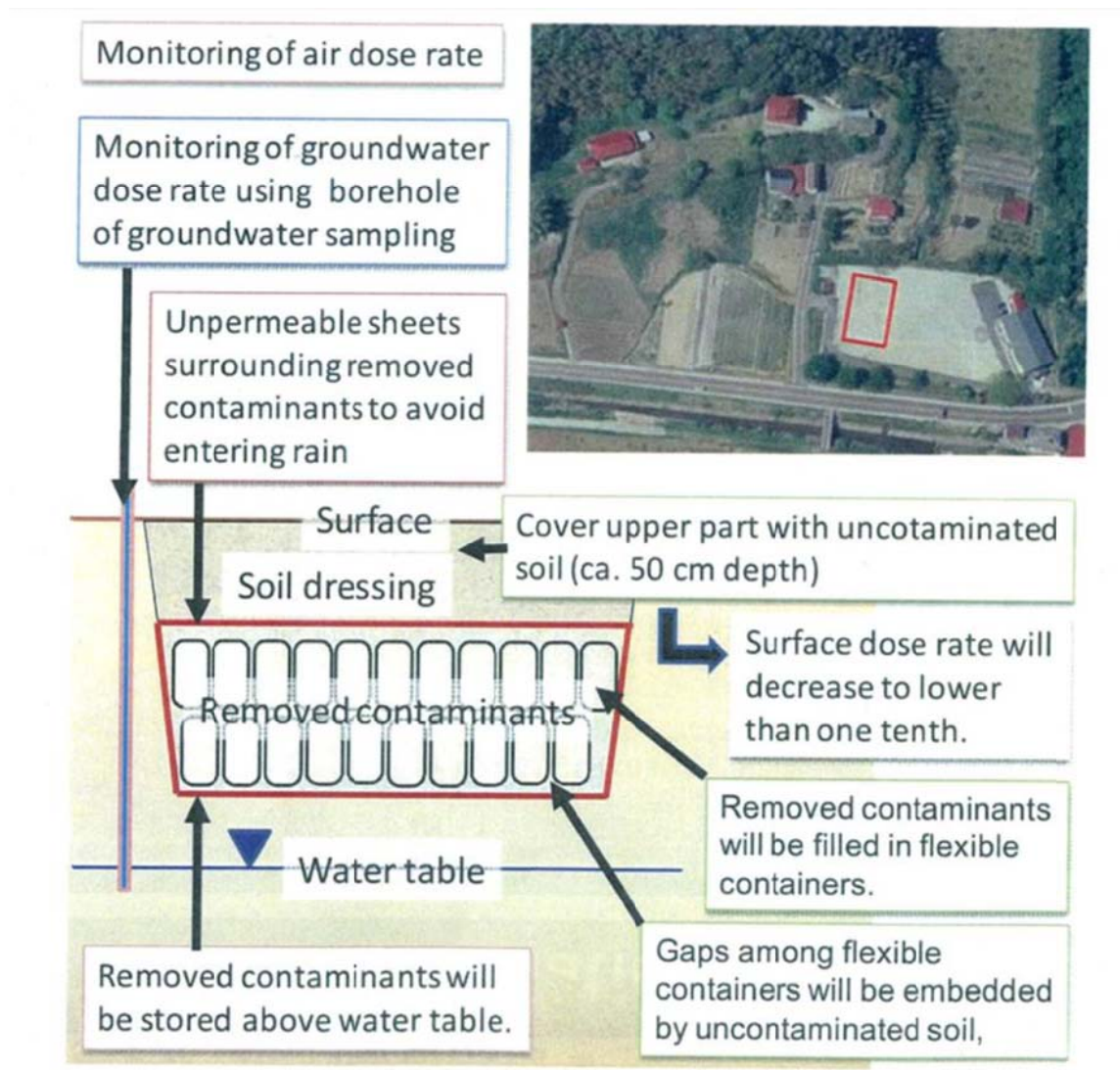
Figure 14: Temporary storage trench for removed contaminated material
