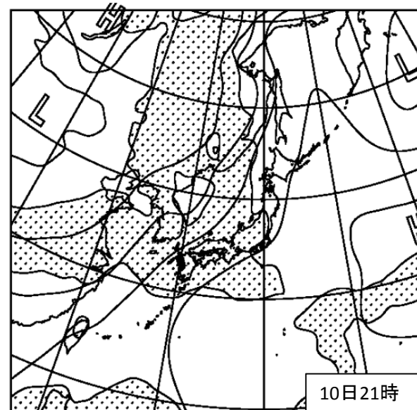
SURFACE PRESS, PRECIP(144-168)
